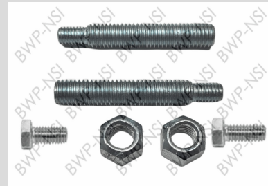
M-3531-KIT Shoulder Stud and Bolt Air Spring Kit
